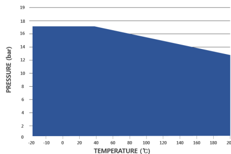
Pressure-Temperature Chart
